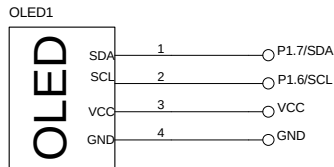
.96" OLED 128X64 GRAPHIC SCREEN WITH SSD1306
