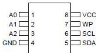
8-Pin SOIC
